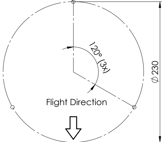
Hole Pattern
